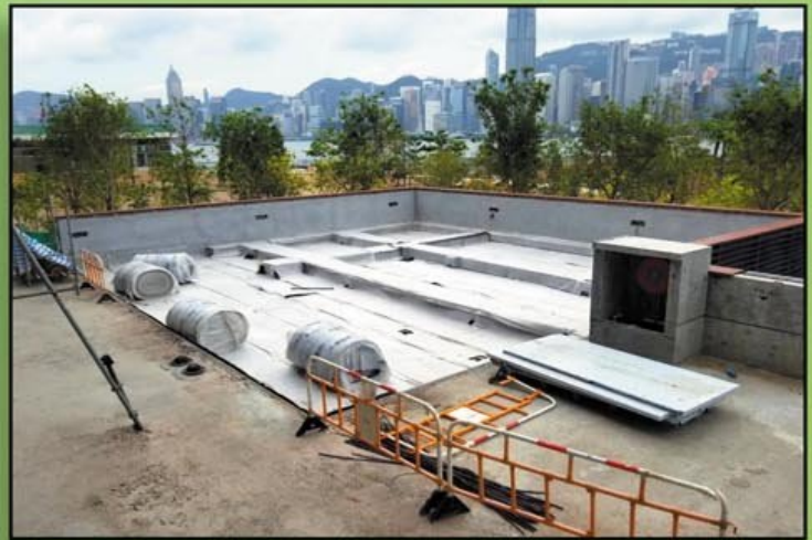
West Kowloon Cultural District Park Geocomposite Planter Drainage, August 2018 西九文化公園花槽排水土工複合材料
