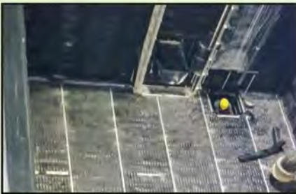
PVC keyed membrane, concrete protection lining at Kai Tak Development pumping station, Nov 2015 混凝土防污保護膜
